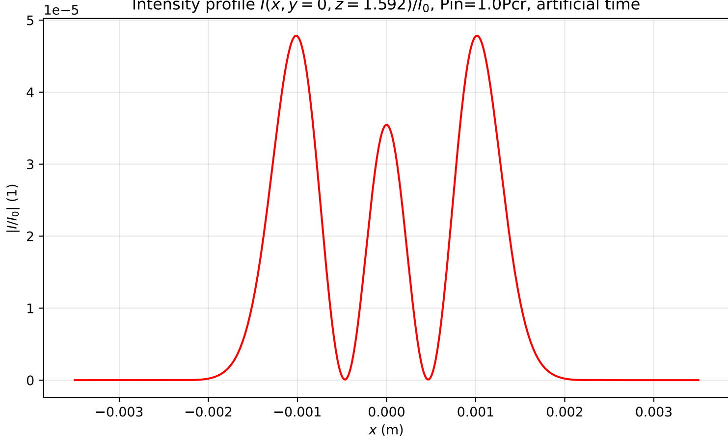
Intensity profile I(x, y = 0, z = 1.592)/I_0 , P_{in}=1.0P_{cr} , artificial time
